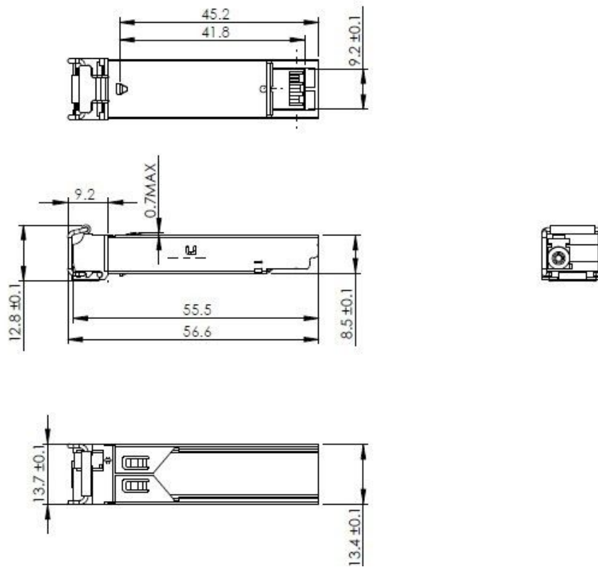
Mechanical Drawing
