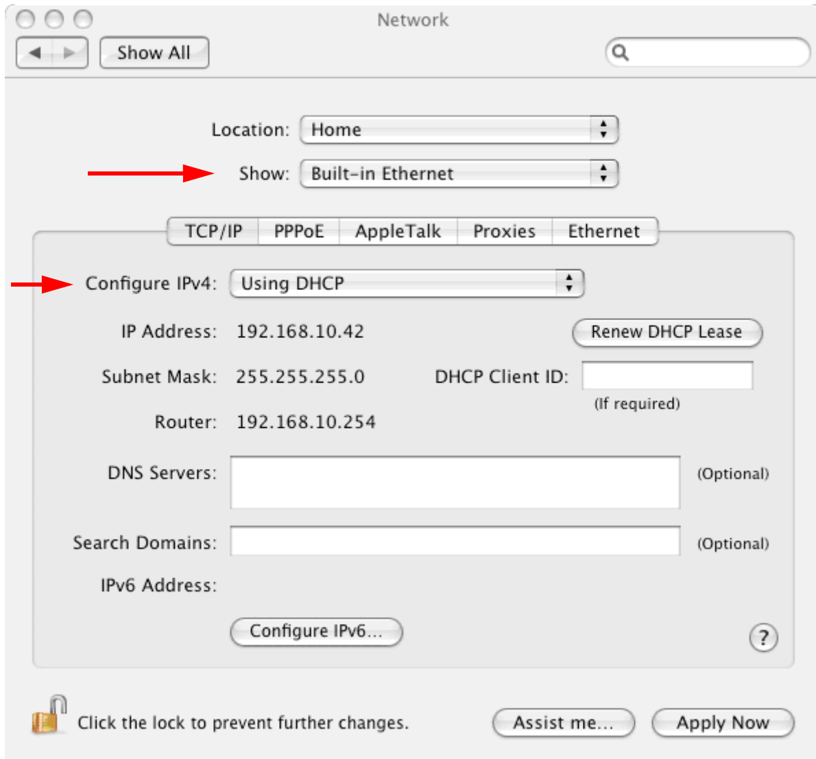
Figure 13 —Configuring Macintosh network settings
