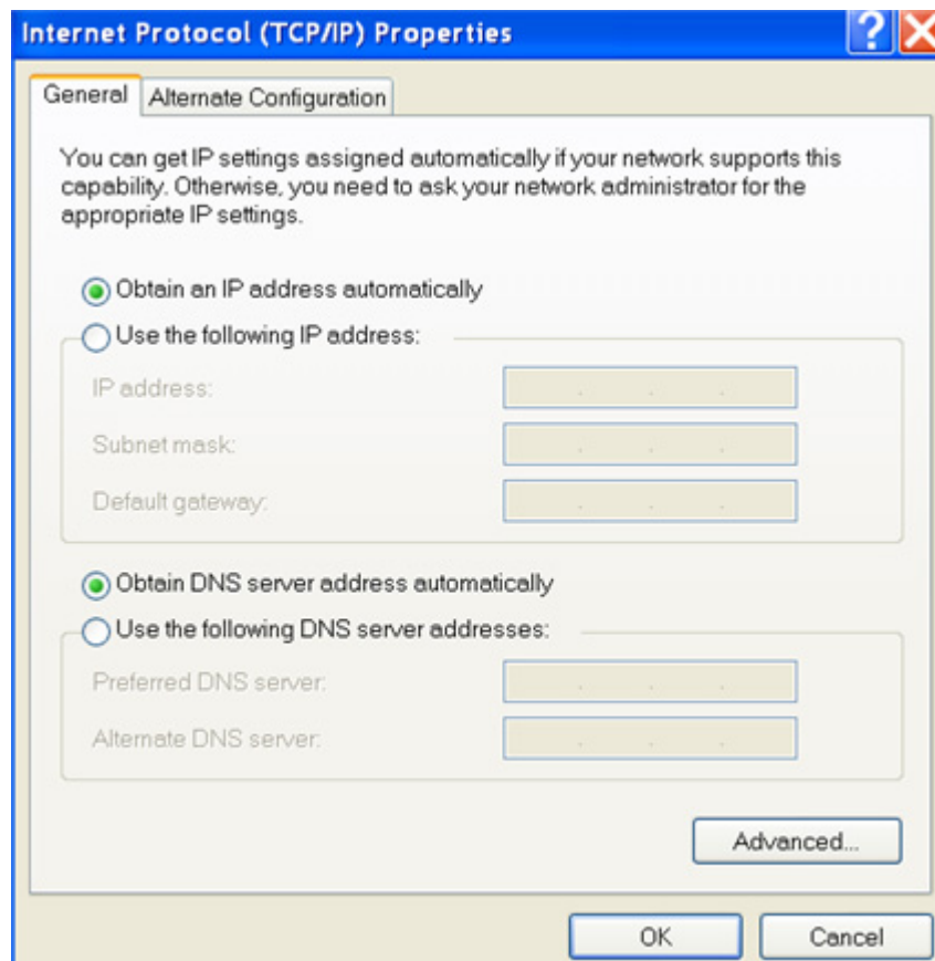
Figure 11 —Internet Protocol (TCP/IP) Properties for Microsoft Windows computers
