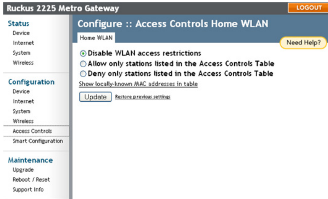
Figure 48—Configuring Access Controls main page
