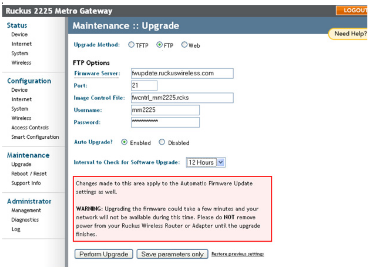
Figure 66—Maintenance :: Upgrade firmware page
