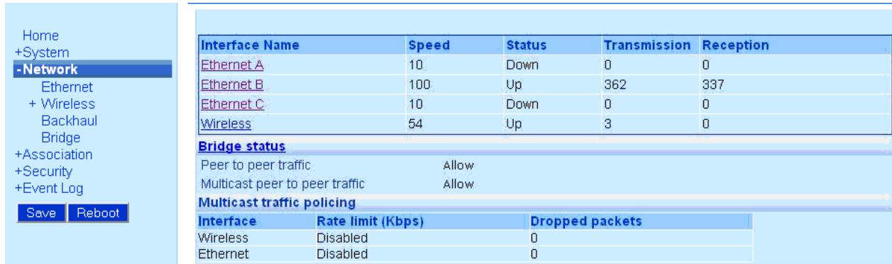
Figure 3.2 Network Interfaces Summary for units with embedded Ethernet Switch
