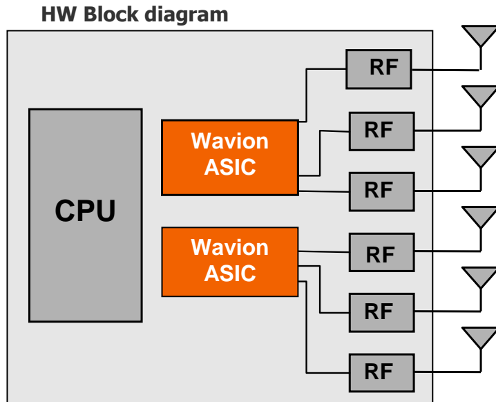
Figure 1.1: Shows the relationship between the WBS-2400 hardware modules.
